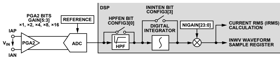
Figure 43. Neutral Current Signal Path
