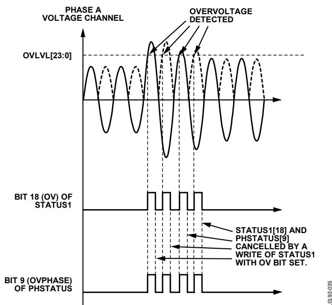
Figure 62. Overvoltage Detection
