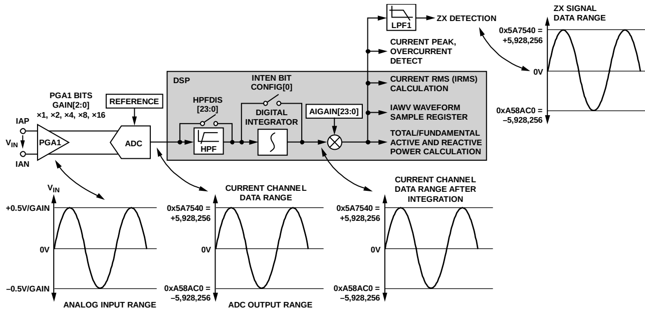
Figure 33. Current Channel Signal Path
