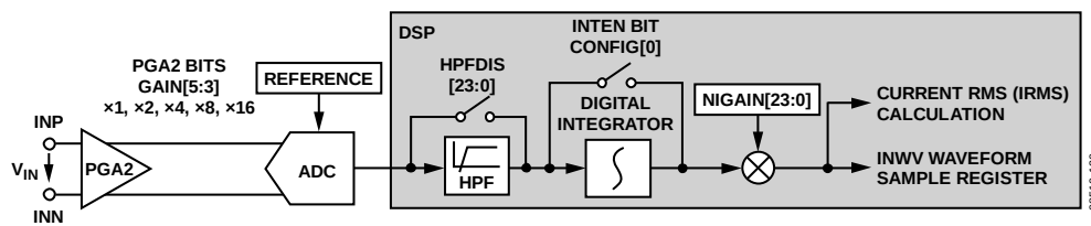
Figure 34. Neutral Current Signal Path (ADE7868, ADE7878 Only)
