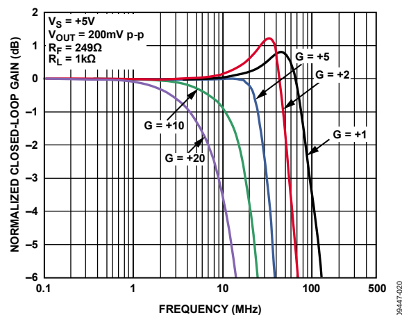
Figure 51. Small Signal Frequency Response at Various Gains
