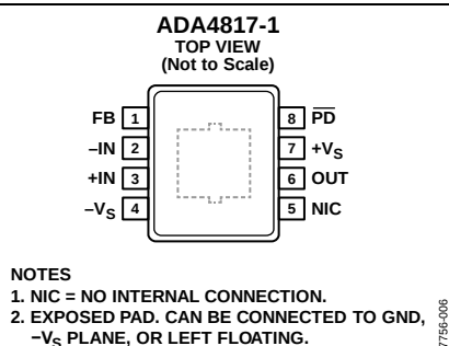
Figure 6. ADA4817-1 Pin Configuration (8-Lead SOIC)
