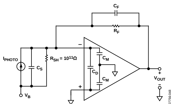
Figure 63. Wideband Photodiode Preamplifier
