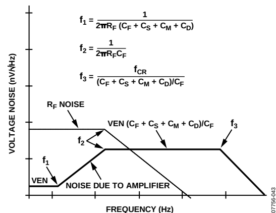
Figure 64. Photodiode Voltage Noise Contributions
