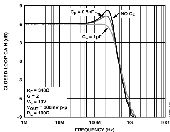
Figure 59. Small Signal Frequency Response vs. Feedback Capacitor (ADA4817-2)
