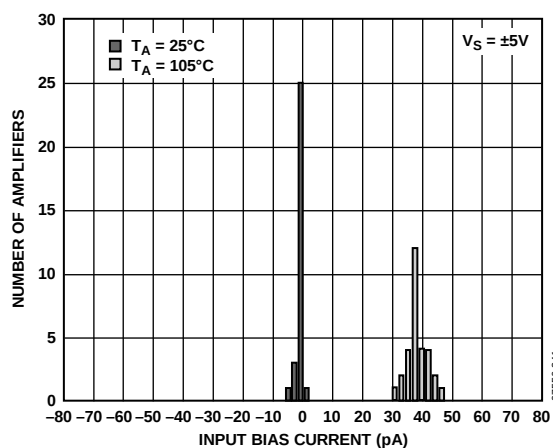
Figure 40. Input Bias Current Histogram over Temperature ( V_S = \pm 5\text{ V} )
