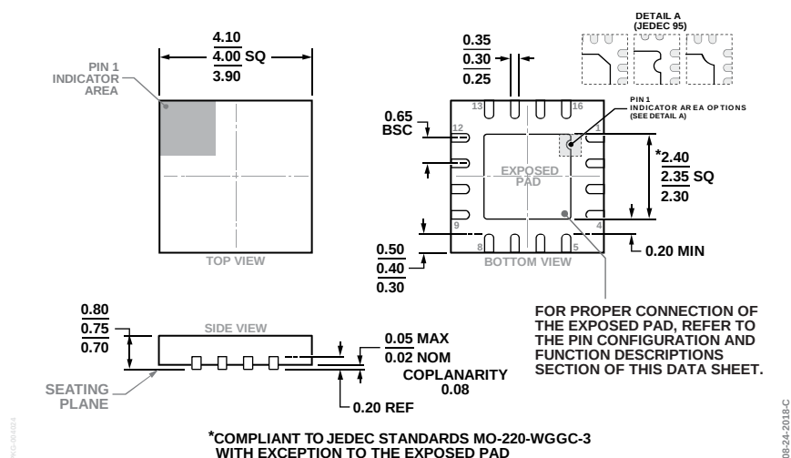
Figure 73.16-Lead Lead Frame Chip Scale Package [LFCSP] 4 mm × 4 mm Body and 0.75 mm Package Height (CP-16-20)
