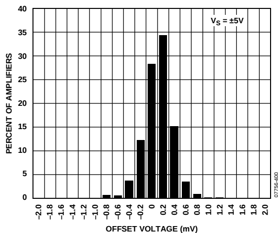
Figure 32. Input Offset Voltage Histogram ( V_S = \pm 5V , LFCSP Only)
