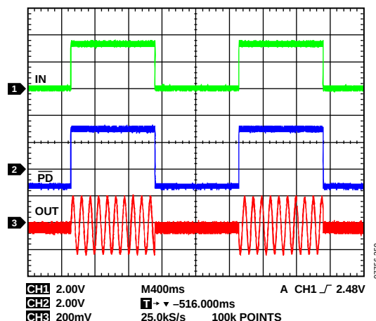
Figure 58. Power-Down Operation
