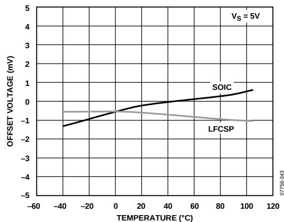
Figure 41. Offset Voltage vs. Temperature ( V_S = 5\text{ V} )
