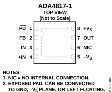
Figure 5. ADA4817-1 Pin Configuration (8-Lead LFCSP)
