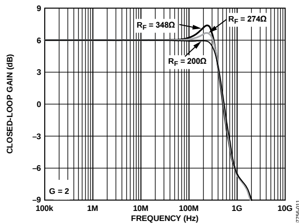
Figure 13. Small Signal Frequency Response for Various R_F
