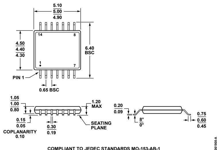
COMPLIANT TO JEDEC STANDARDS MO-153-AB-1 Figure 86. 14-Lead Thin Shrink Small Outline Package [TSSOP] (RU-14) Dimensions shown in millimeters
