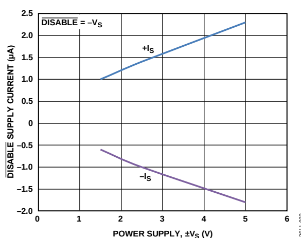
Figure 27. DISABLE Supply Current vs. Power Supply, \pm V_S
