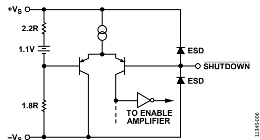
Figure 53. Shutdown Circuit
