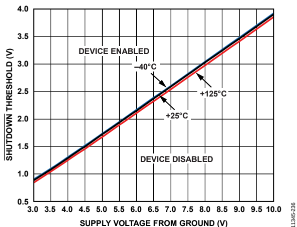
Figure 43. \overline{\text{SHUTDOWN}} Threshold vs. Supply Voltage from Ground for Various Temperatures
