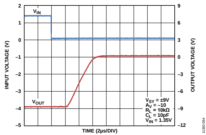
Figure 53. Negative Overload Recovery
