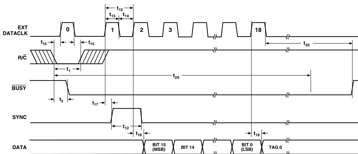
Figure 7. Conversion and Read Timing for Reading Previous Conversion Results During a Conversion Using External Discontinuous Data Clock ( \overline{\text{EXT/INT}} Set to Logic High, \overline{\text{CS}} Set to Logic Low)
