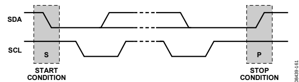
Figure 31. Start and Stop Conditions
