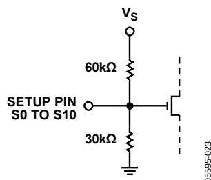
Figure 22. Setup Pin ( S_0 to S_{10} ) Equivalent Circuit
