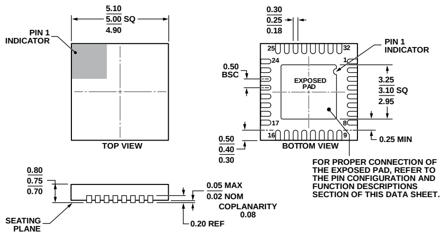
Figure 64. 32-Lead Lead Frame Chip Scale Package [LFCSP_WQ] 5 x 5 mm Body, Very Very Thin Quad (CP-32-7) Dimensions shown in millimeters
