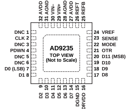
Figure 4. 32-Lead LFCSP Pin Configuration
