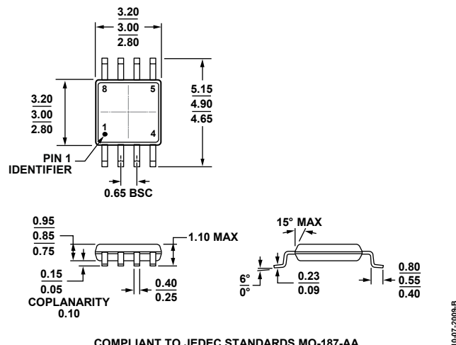
Figure 67. 8-Lead Mini Small Outline Package [MSOP] (RM-8)
