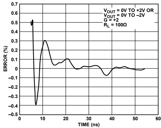
Figure 18. Settling Time
