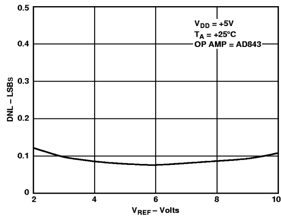
Figure 5. Differential Nonlinearity Error vs. V_{REF} (Normal Mode)
