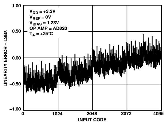
Figure 9. All Codes Linearity in Biased Mode ( V_{DD} = +3.3 V )
