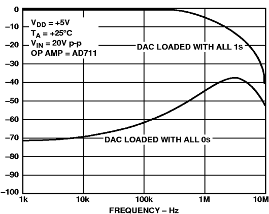
Figure 12. Multiplying Frequency Response vs. Digital Code
