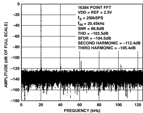
Figure 12. FFT Plot
