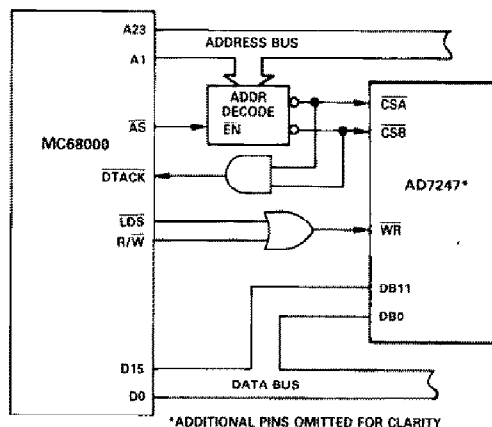
Figure 12. AD7247 to MC68000 Interface
