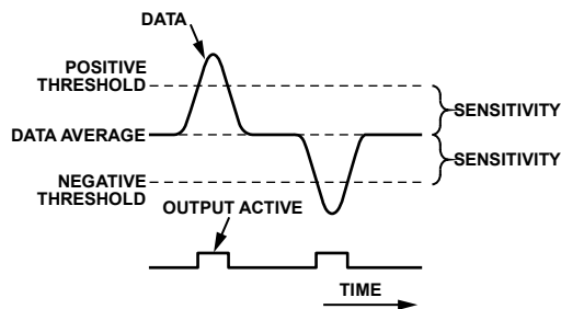
Figure 30. Threshold Sensitivity
