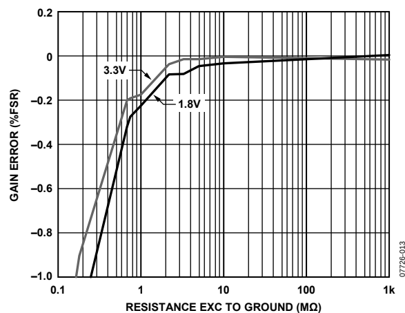
Figure 13. Capacitance Input Gain Error vs. Resistance EXC to GND, V_{DD} = 1.8\text{ V} and 3.3\text{ V} , CIN to EXC = 9\text{ pF}
