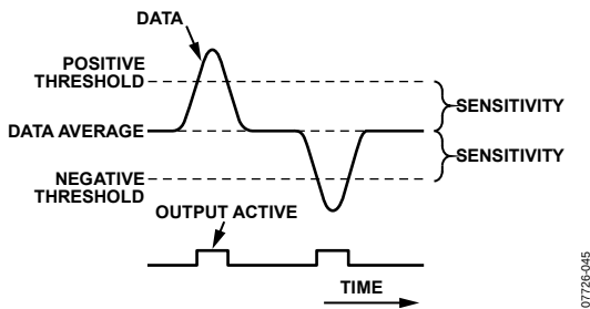
Figure 37. Threshold Sensitivity
