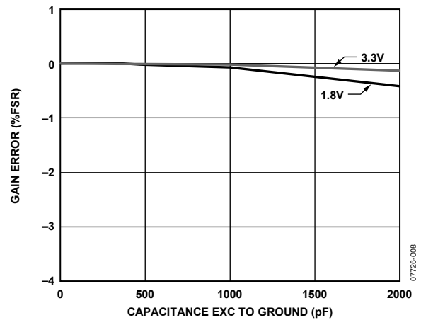
Figure 8. Capacitance Input Gain Error vs. Capacitance C_{EXC} to GND, V_{DD} = 1.8V and 3.3V , C_{IN} to C_{EXC} = 3pF
