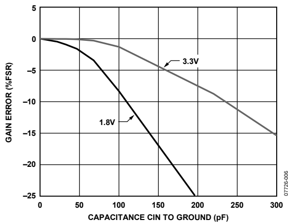
Figure 6. Capacitance Input Gain Error vs. Capacitance C_{IN} to GND, V_{DD} = 1.8V and 3.3V , C_{IN} to C_{EXC} = 9pF
