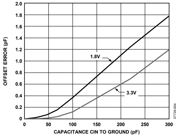
Figure 4. Capacitance Input Offset Error vs. Capacitance C_{IN} to GND, V_{DD} = 1.8V and 3.3V , EXC Pin Open Circuit
