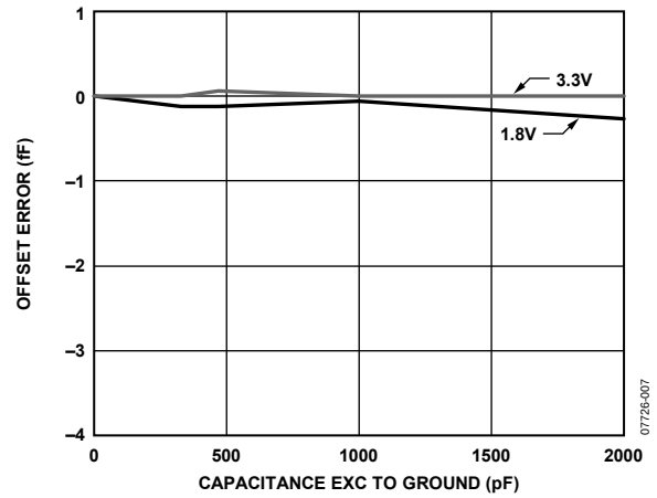
Figure 7. Capacitance Input Offset Error vs. Capacitance C_{EXC} to GND, V_{DD} = 1.8V and 3.3V , C_{IN} Pin Open Circuit
