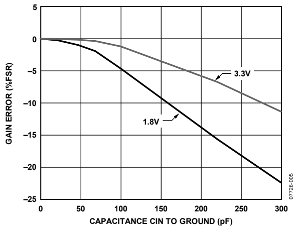
Figure 5. Capacitance Input Gain Error vs. Capacitance C_{IN} to GND, V_{DD} = 1.8V and 3.3V , C_{IN} to C_{EXC} = 3pF
