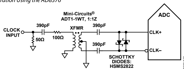
Figure 47. Transformer-Coupled Differential Clock (Up to 200 MHz)
