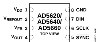
Figure 5. LFCSP Pin Configuration
