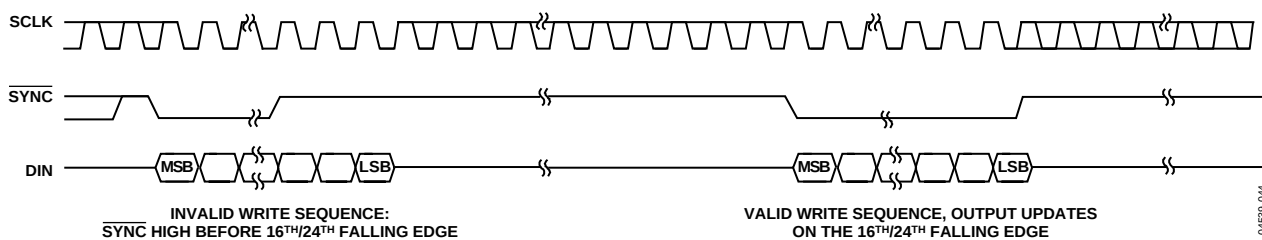
Figure 44. \overline{\text{SYNC}} Interrupt Facility
