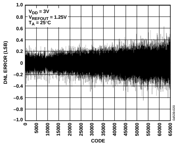
Figure 15. DNL—AD5660-1
