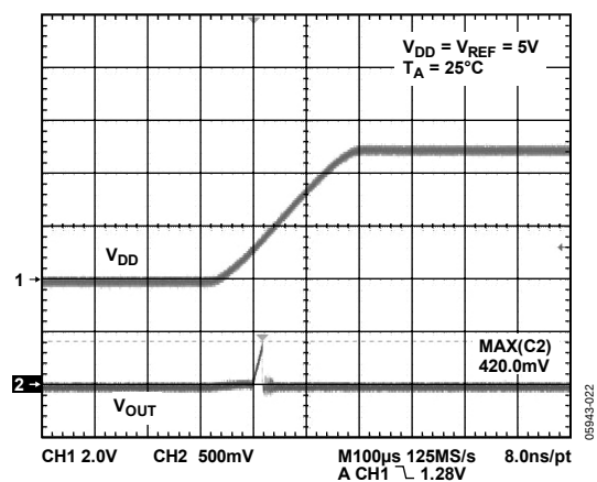
Figure 20. Power-On Reset to 0\text{ V}
