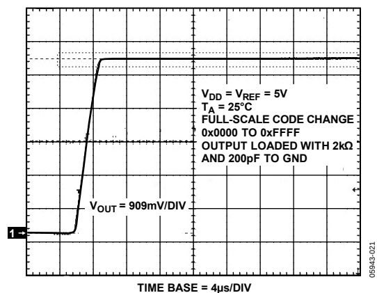
Figure 19. Full-Scale Settling Time, 5\text{ V}
