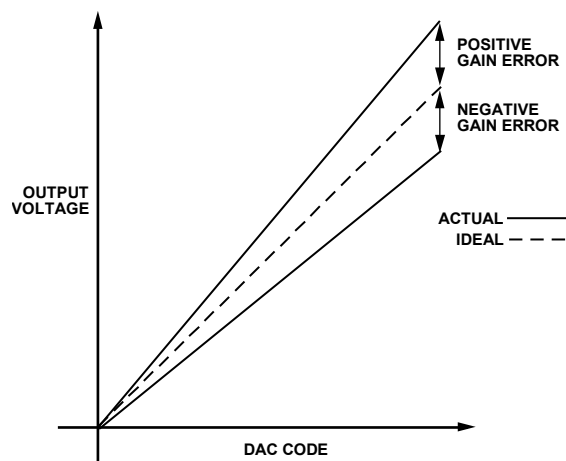
Figure 11. Gain Error
