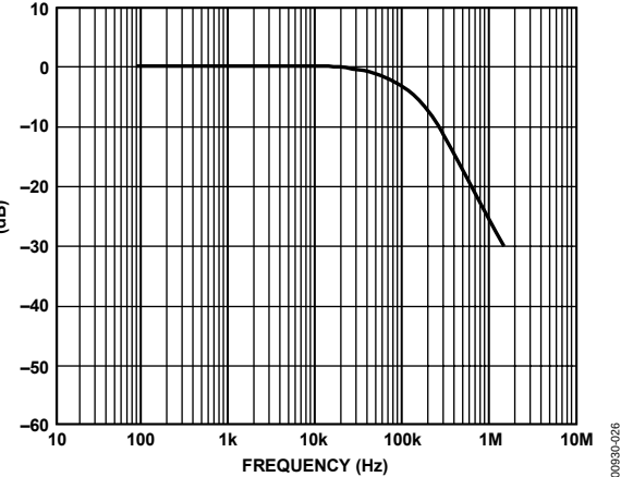
Figure 24. Multiplying Bandwidth (Small-Signal Frequency Response)
