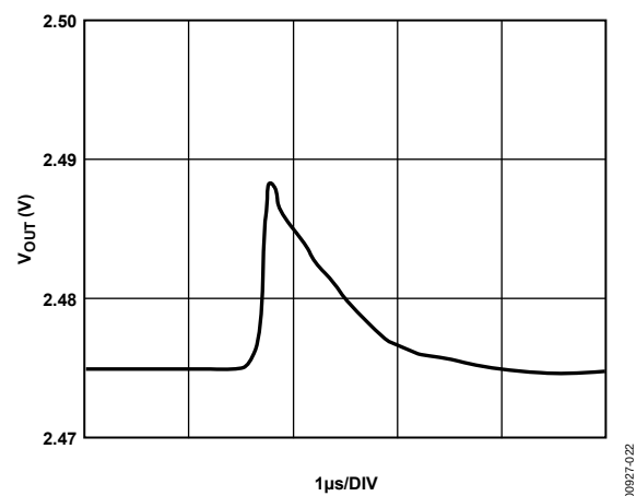
Figure 22. Major-Code Transition
