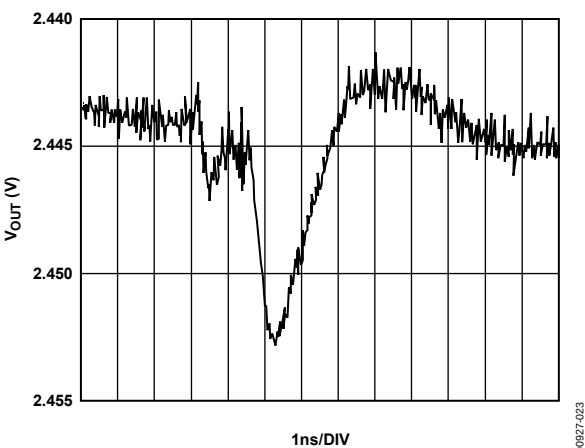
Figure 23. Digital Feedthrough
