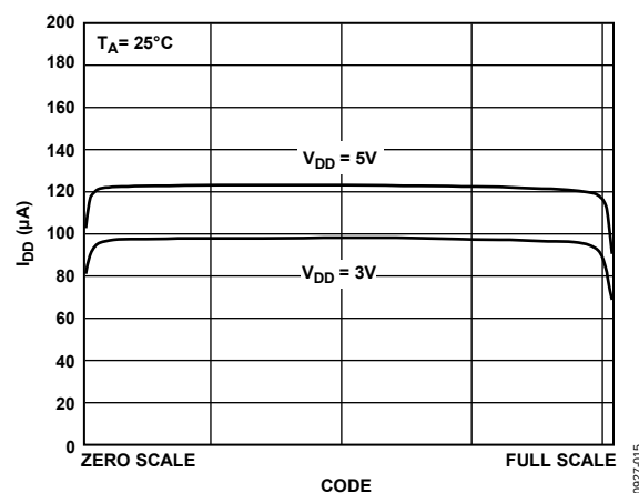
Figure 15. Supply Current vs. Code
