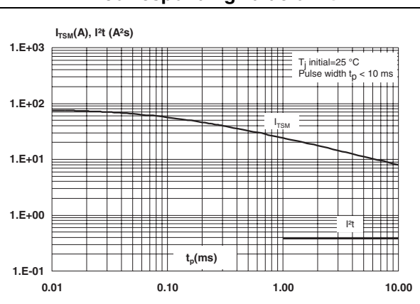
Figure 7. Non repetitive surge peak on-state current for a sinusoidal pulse, and corresponding value of I²t
