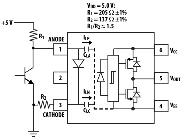
Figure 32 Recommended High-CMR Drive Circuit for the ACPL-P343/W343
