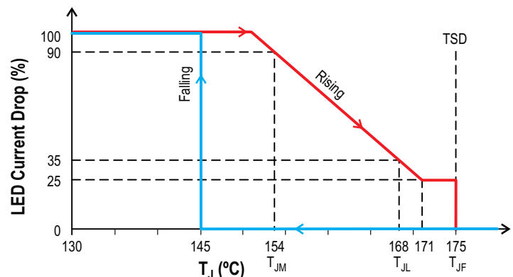
Figure 8: Output Current Foldback Based on Rising T_J Output current changed by DC current control; when temperature exceeds 175^{\circ}\text{C} (typ), the IC turns off due to TSD function, and turns on again at 145^{\circ}\text{C} ( 30^{\circ}\text{C} (typ)) hysteresis.
