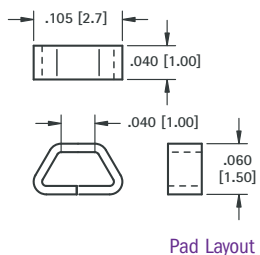
Pad Layout
