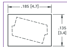
Pad Layout
