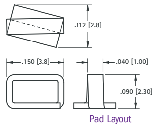
Pad Layout
