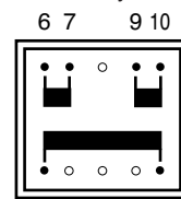
Primary winding
