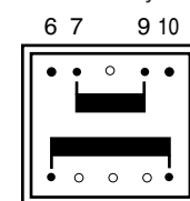
Primary winding
