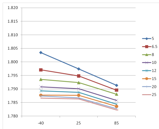
Fig. 18: Temperature Regulation 1.8V OUT (±1% Vo window)
