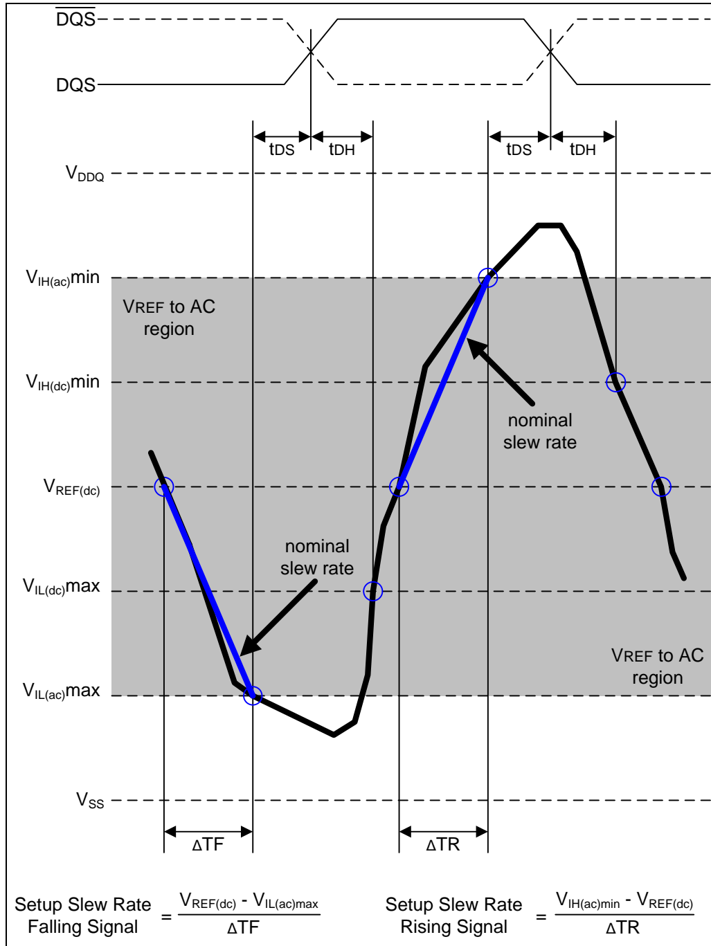
Figure 24 – Illustration of nominal slew rate for t_{\text{DS}} (differential DQS, \overline{\text{DQS}} )
