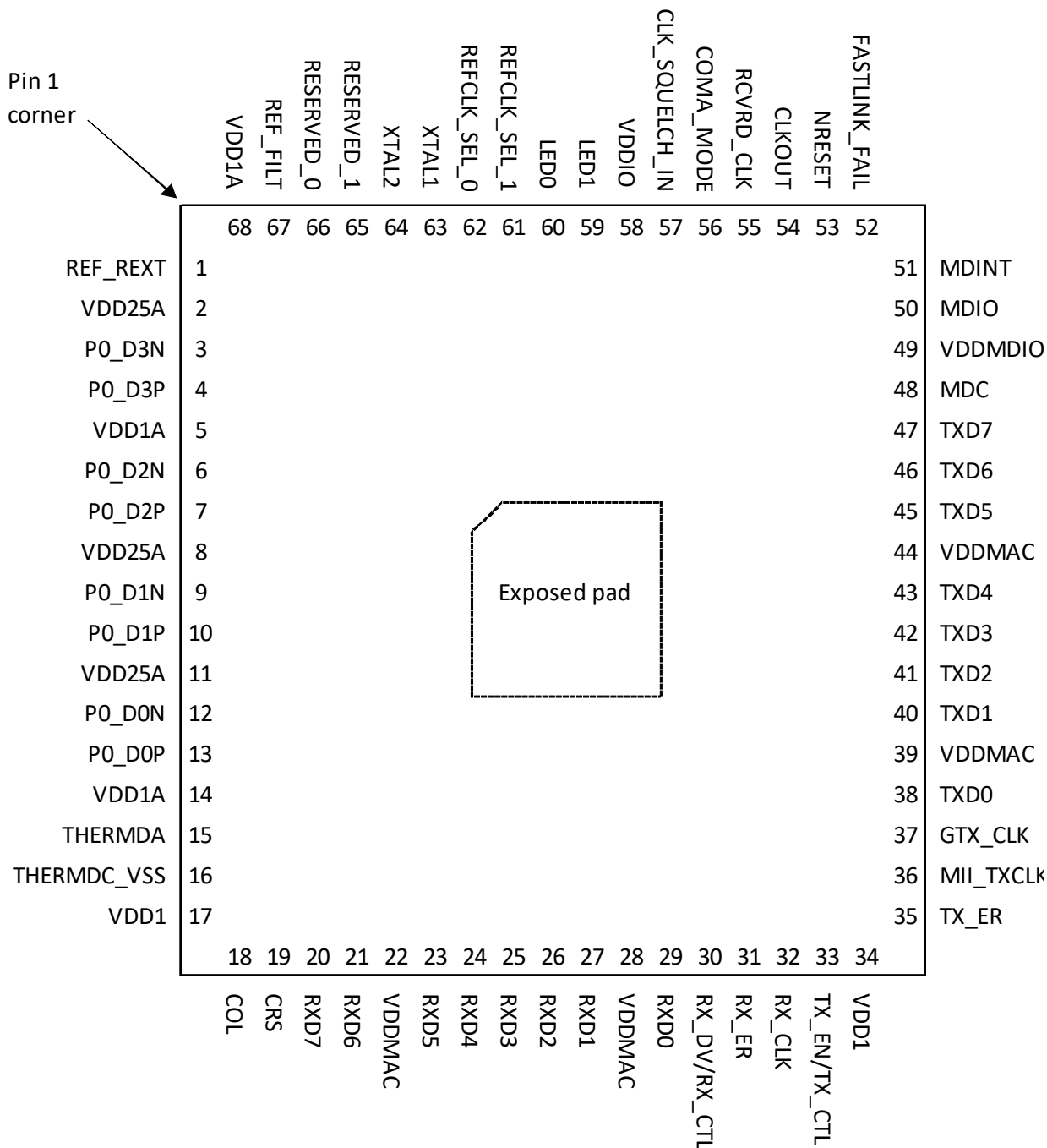
Figure 35 • Pin Diagram
