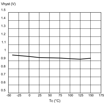
Figure 16. Input hysteresis voltage
