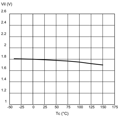
Figure 18. Input low level
