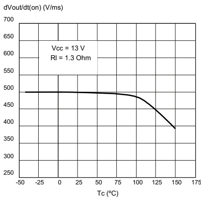
Figure 10. Turn-on voltage slope
