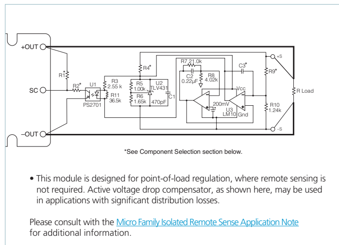
Figure 12 — Voltage-drop compensation
