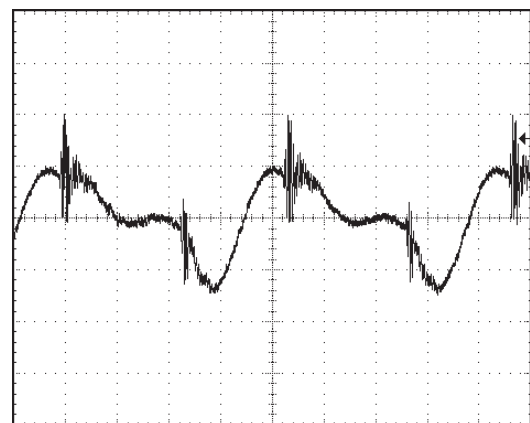
Output Ripple and Noise (PARD)
