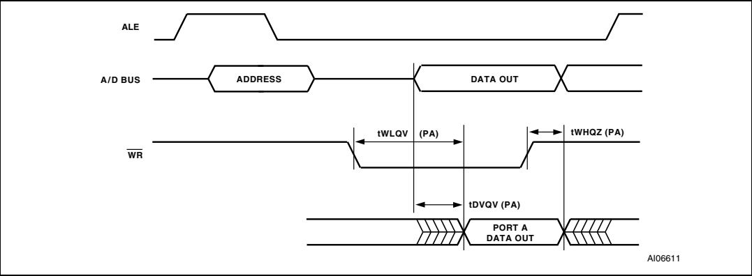
Figure 78. Peripheral I/O Write timing
