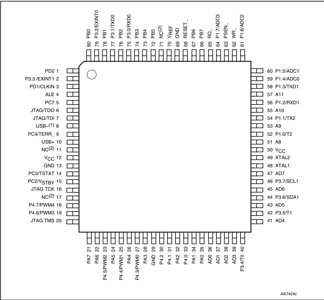
Figure 3. TQFP80 connections
