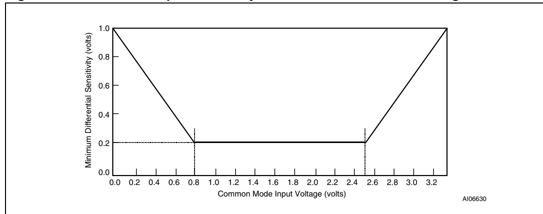
Figure 40. Differential input sensitivity over entire common mode range
