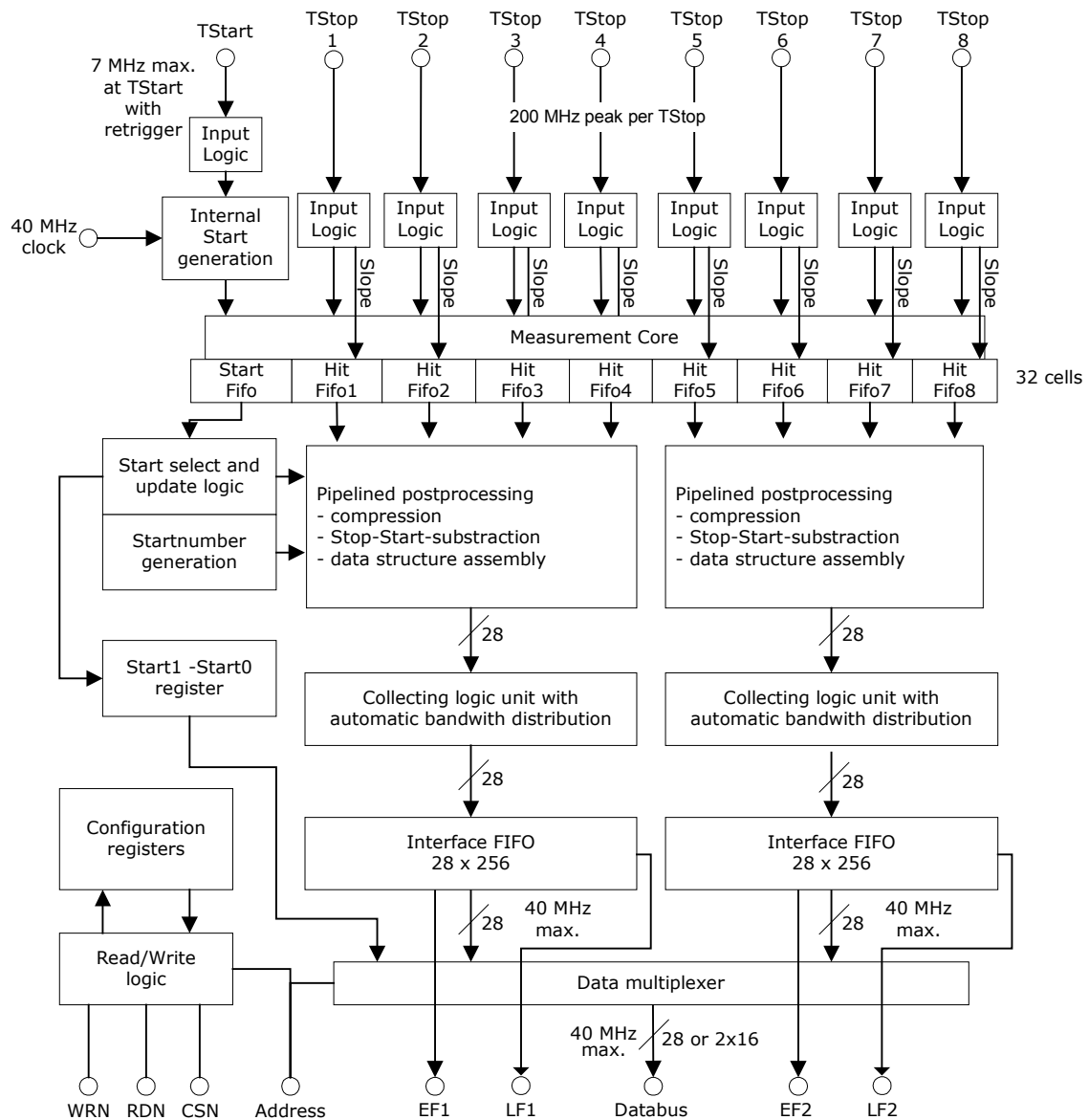
Figure 16: Block diagram
