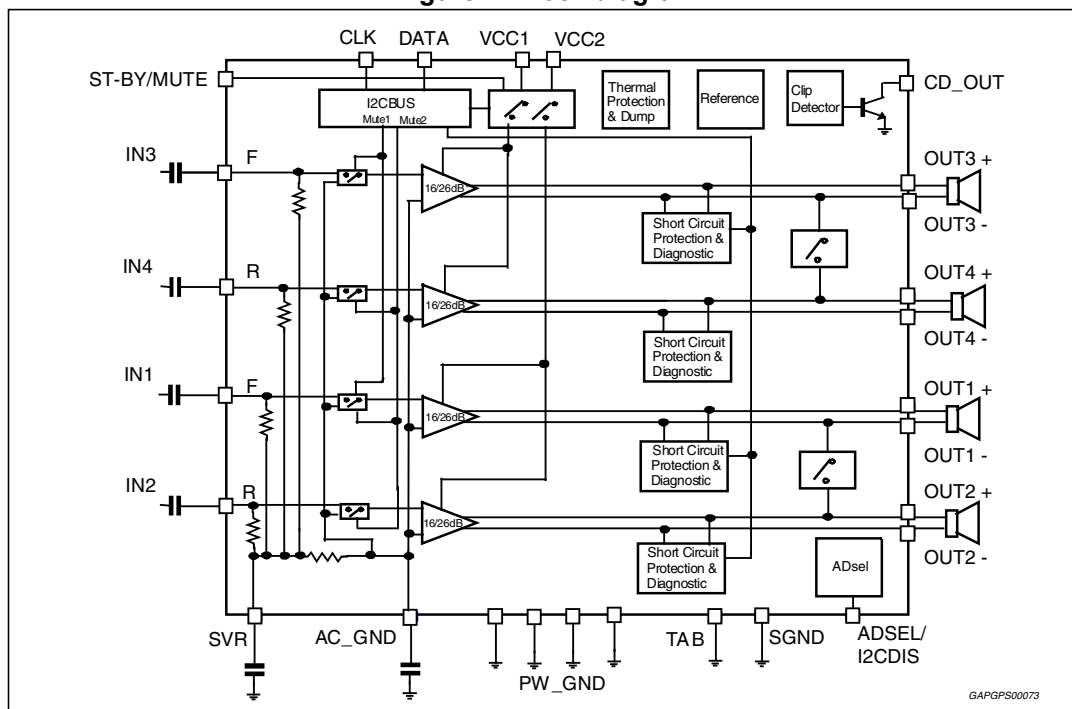
Figure 2. Block diagram
