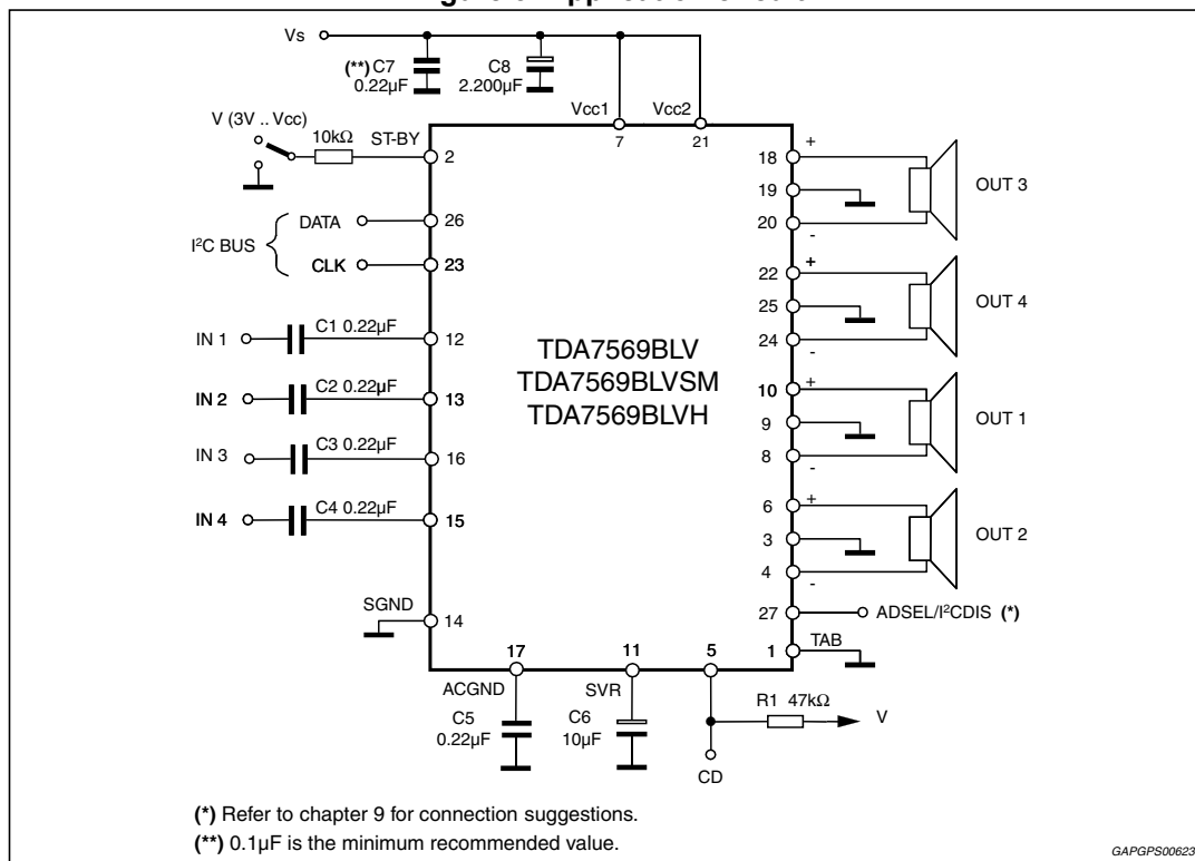
Figure 3. Application circuit
