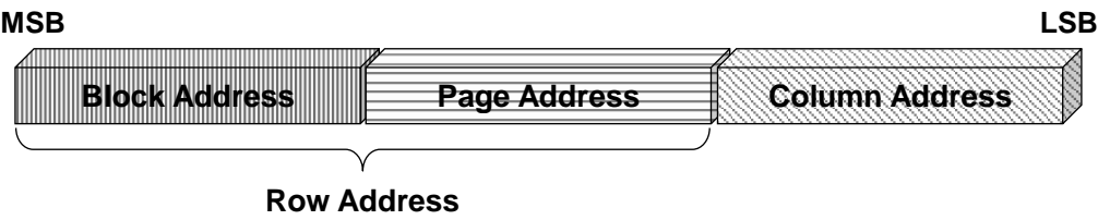
Figure 4. Addressing
