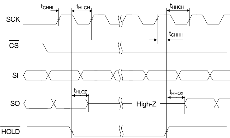
Figure 8. Hold Timing
