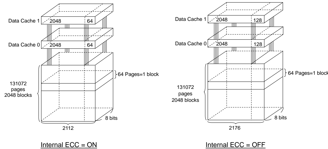
Figure 3. Cell Layout
