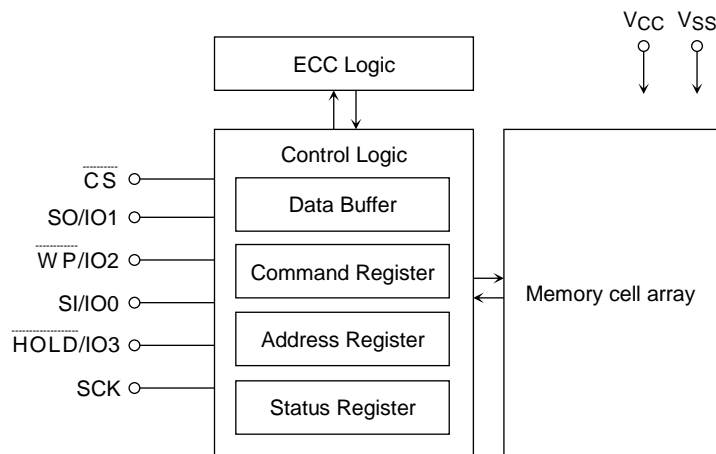
Figure 2. Block Diagram
