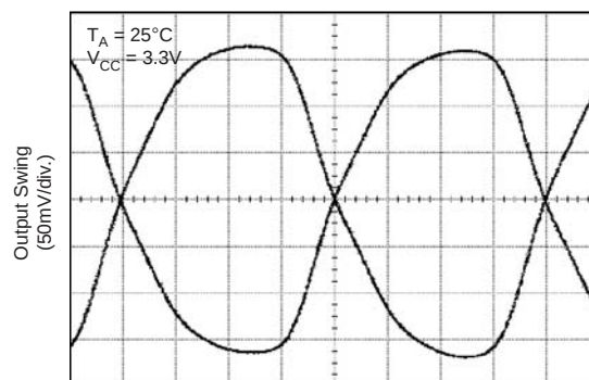
622MHz Output
