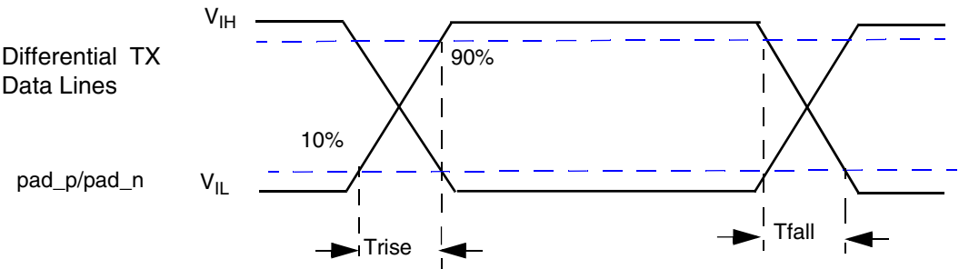
Figure 32. Rise/fall time
