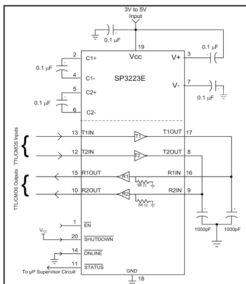
Figure 14. Loopback Test Circuit for RS-232 Driver
