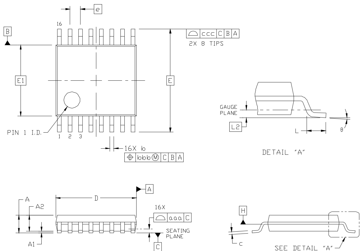
Figure 15. 16-Pin TSSOP
