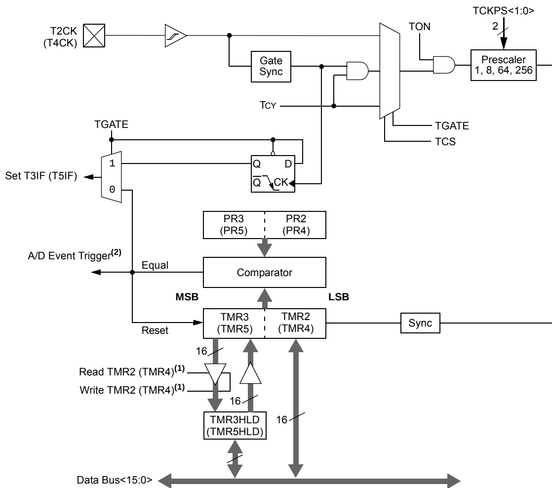
FIGURE 13-1: TIMER2/3 AND TIMER4/5 (32-BIT) BLOCK DIAGRAM
