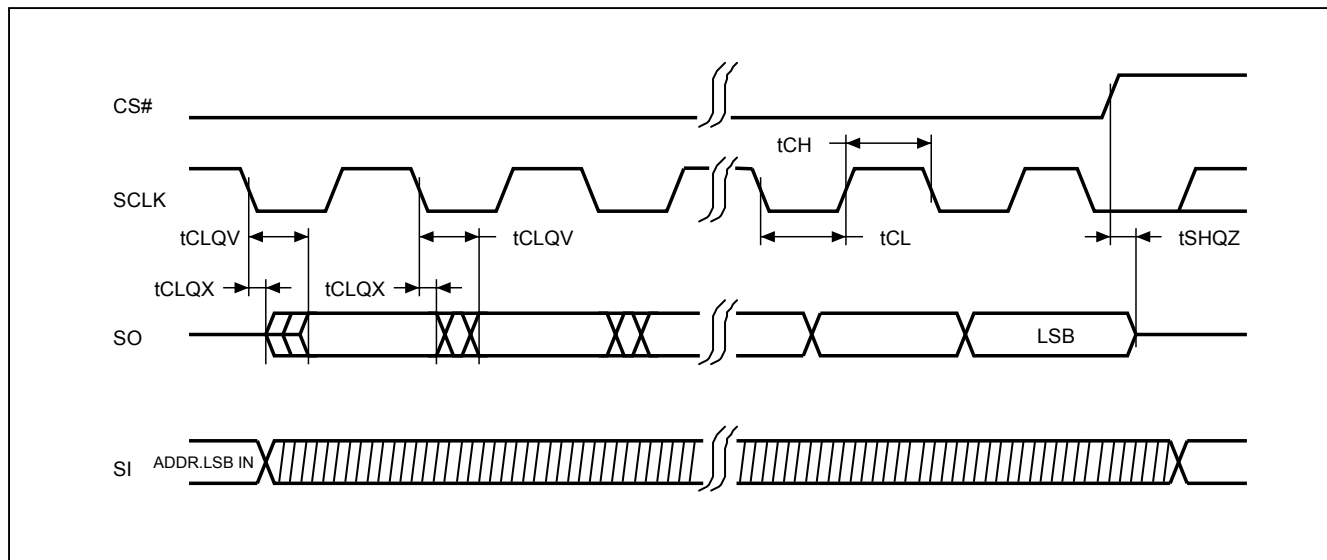
Figure 43. Output Timing
