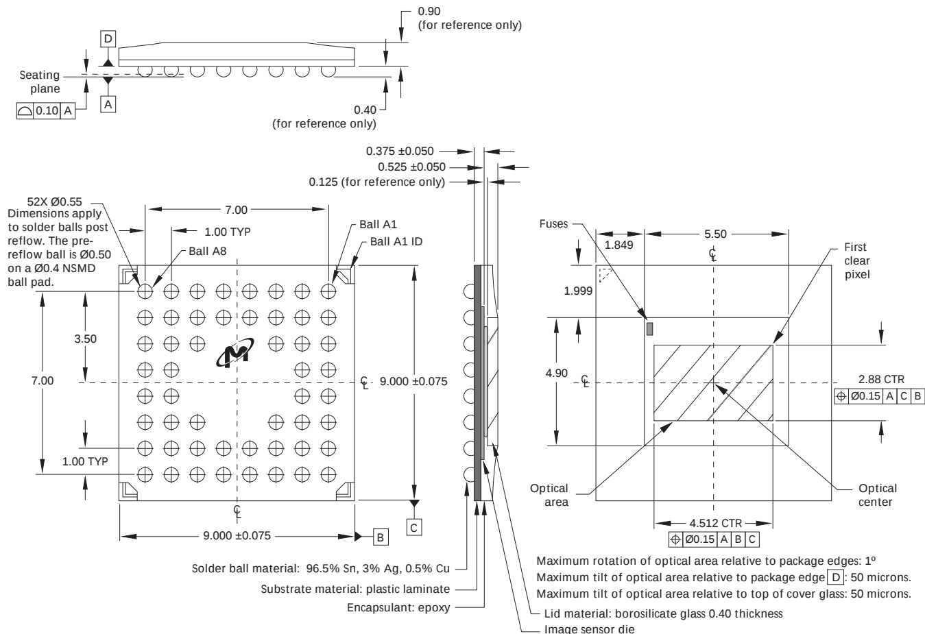
Figure 45: 52-Ball IBGA
