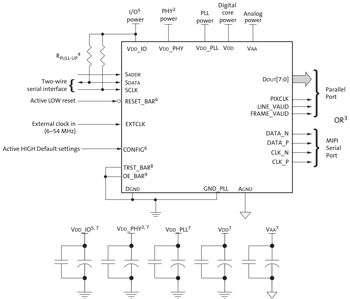
Figure 2: Typical Configuration
