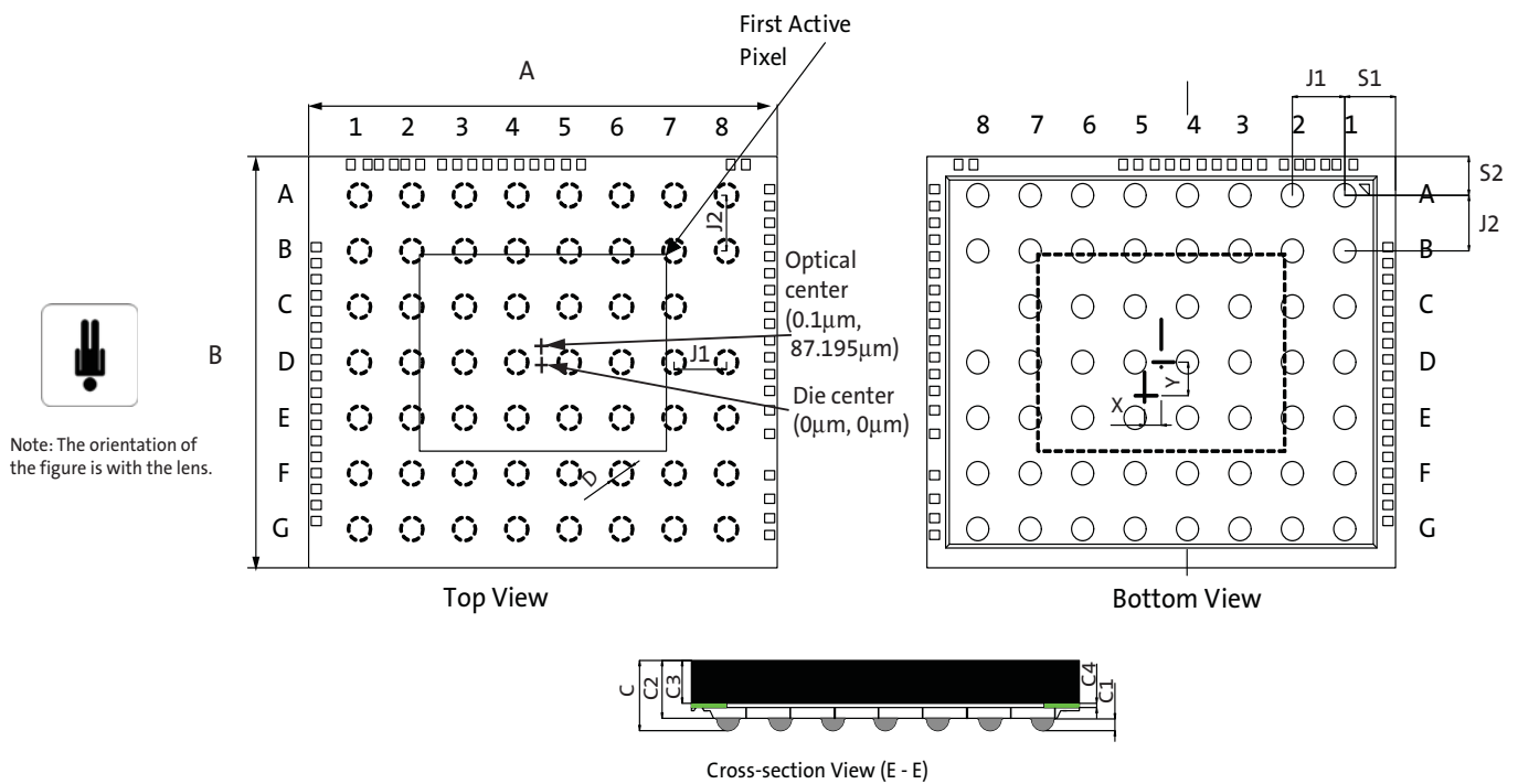
Figure 38: Package Mechanical Drawing
