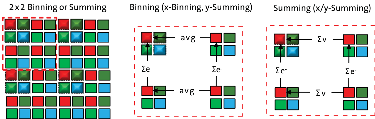
Figure 20: Pixel Readout (Column and Row Binning)
