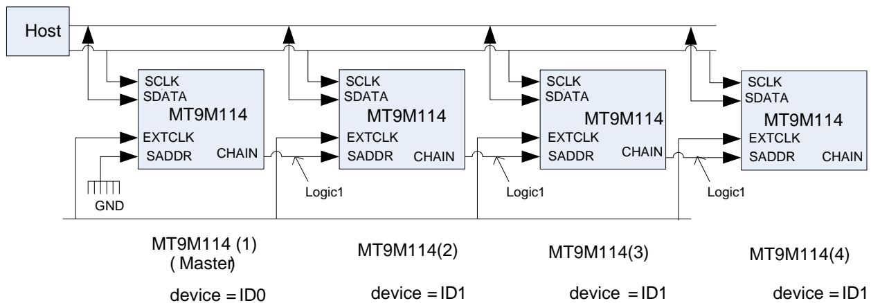
Figure 27: Multi-Camera Connection
