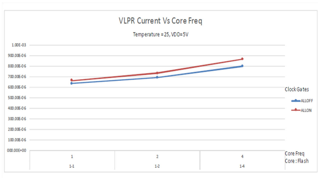
Figure 10. VLPR mode supply current vs. core frequency
