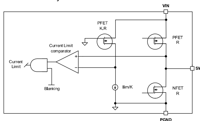
Figure 5. Current-Limit Detail
