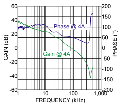
V_{IN} = 5.0V, V_{OUT} = 1.2V
