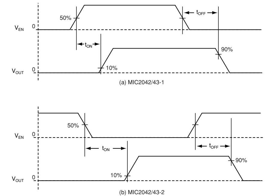
Figure 1. Turn-On/Turn-Off Delay
