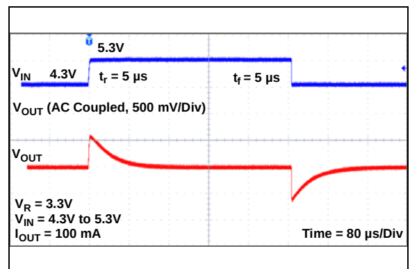
FIGURE 2-47: Dynamic Line Response.
